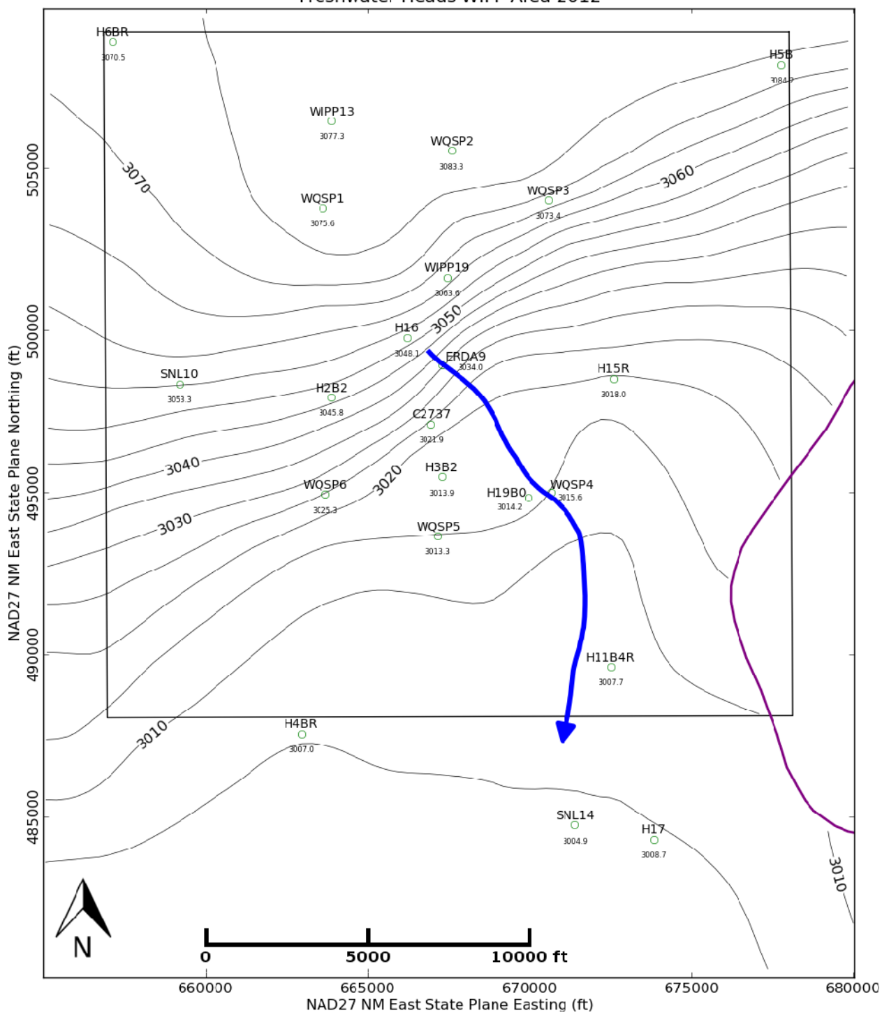
Figure 2.16. February 2012 modeled Culebra potentiometric surface of the immediate WIPP vicinity (DOE 2013c) generated using ensemble average distributed aquifer parameters from the SNL Culebra flow model used in performance assessment baseline calculation for CRA-2009; see Kuhlman (2010b).
