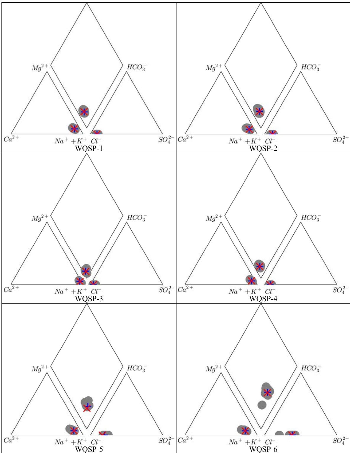
Figure 2.13. Piper diagrams of all data collected from WQSP-1 through WQSP-6. The plots show both historical data (gray areas) and results from rounds 34 (primary = blue star and duplicate = red star).
