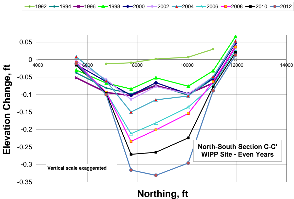
Figure 2.10. East-West subsidence profile C-C'.
