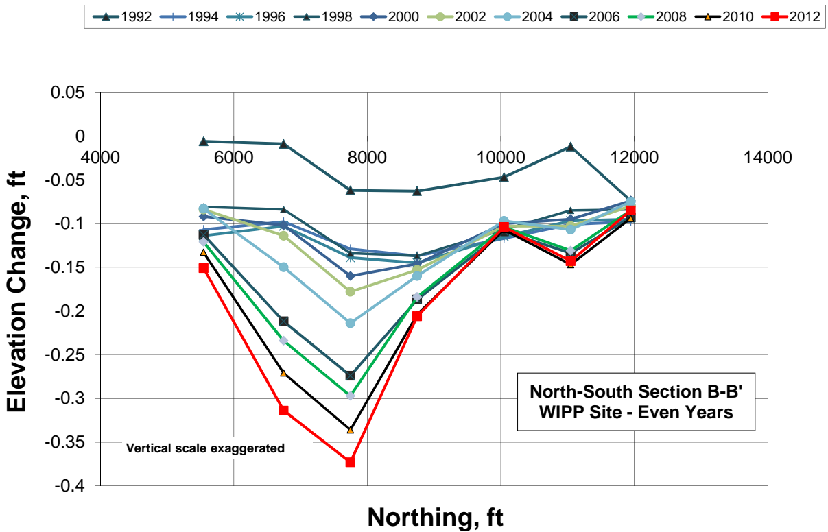
Figure 2.9. North-South subsidence profile B-B'.
